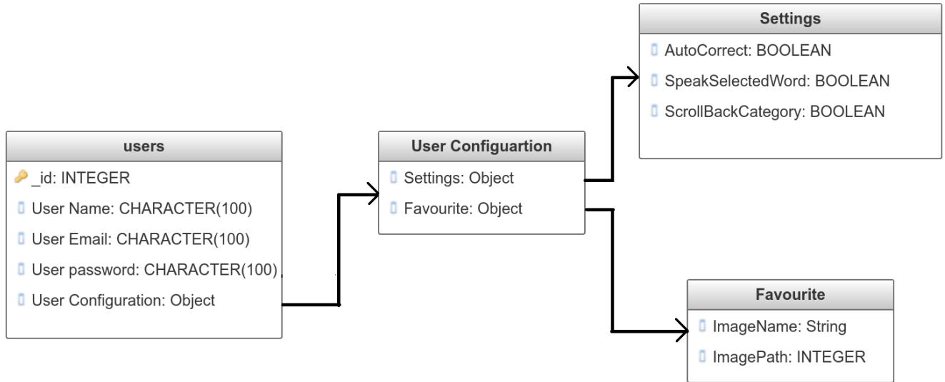
Figure 2.4: System Cloud NoSQL database schema structure
