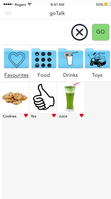
Figure 5.2.1: Favourites Category
