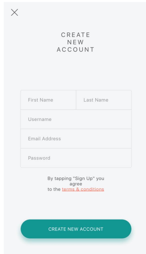
Figure 3.1.2: Registration Screen
