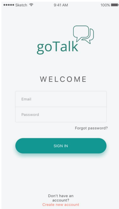
Figure 3.1.1: Login Screen
