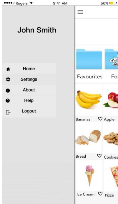
Figure 5.3.1: Menu Window
