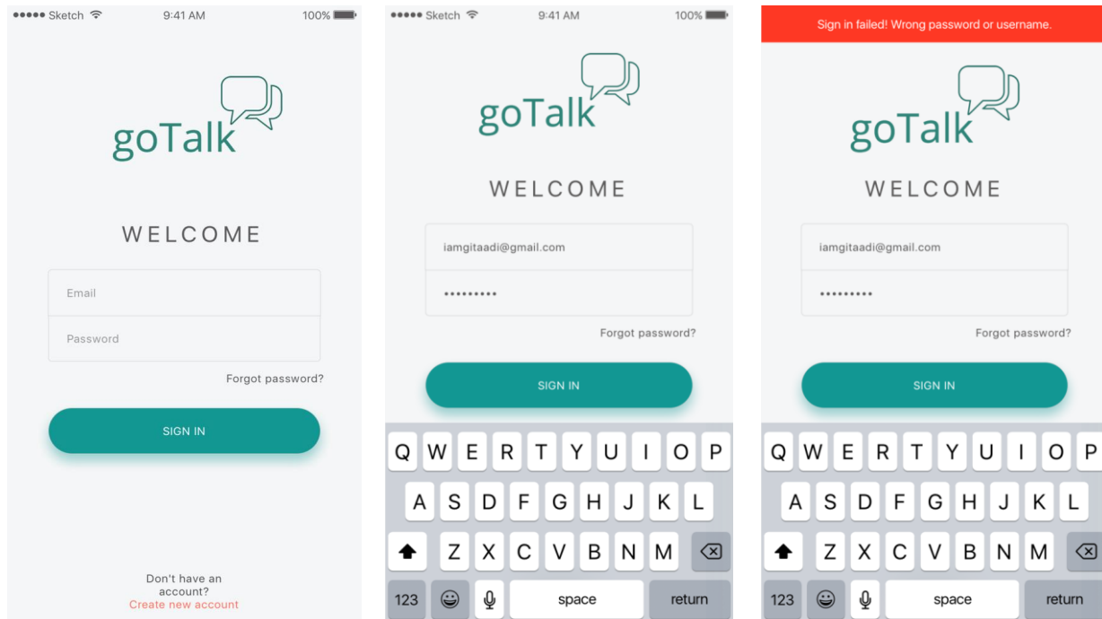
Figure 5.1.1: Login
