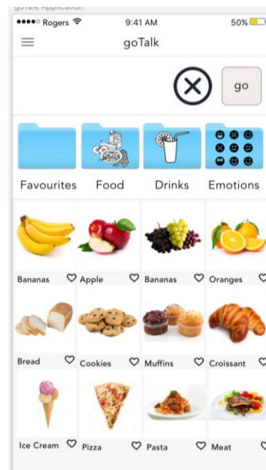
Figure 3.8: Categories Row
