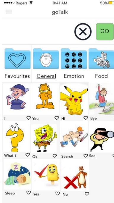
Figure 5.2.2: General Category
