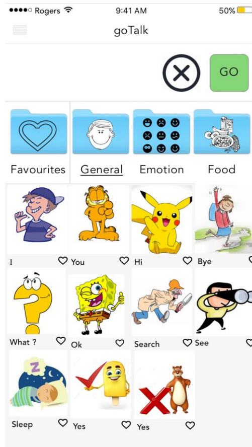
Figure 3.2: Main Screen
