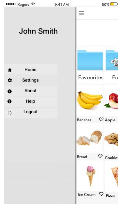
Figure 3.3.2: Menu Window
