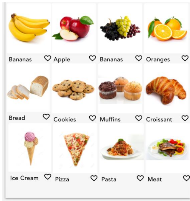
Figure 3.7: Pictographic Buttons
